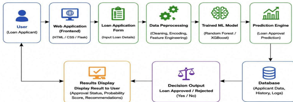
Figure 1: Architecture and data flow of the Smart Lender loan prediction system
